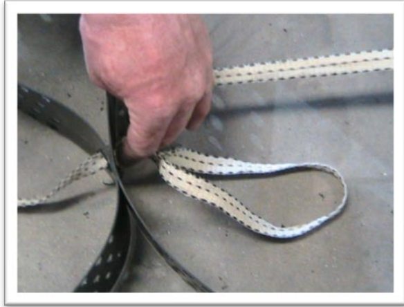
8. Make loop at Envirogrid tendon hole.
