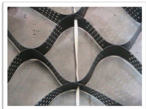
6. View of tendon going thru the EnviroGrid
